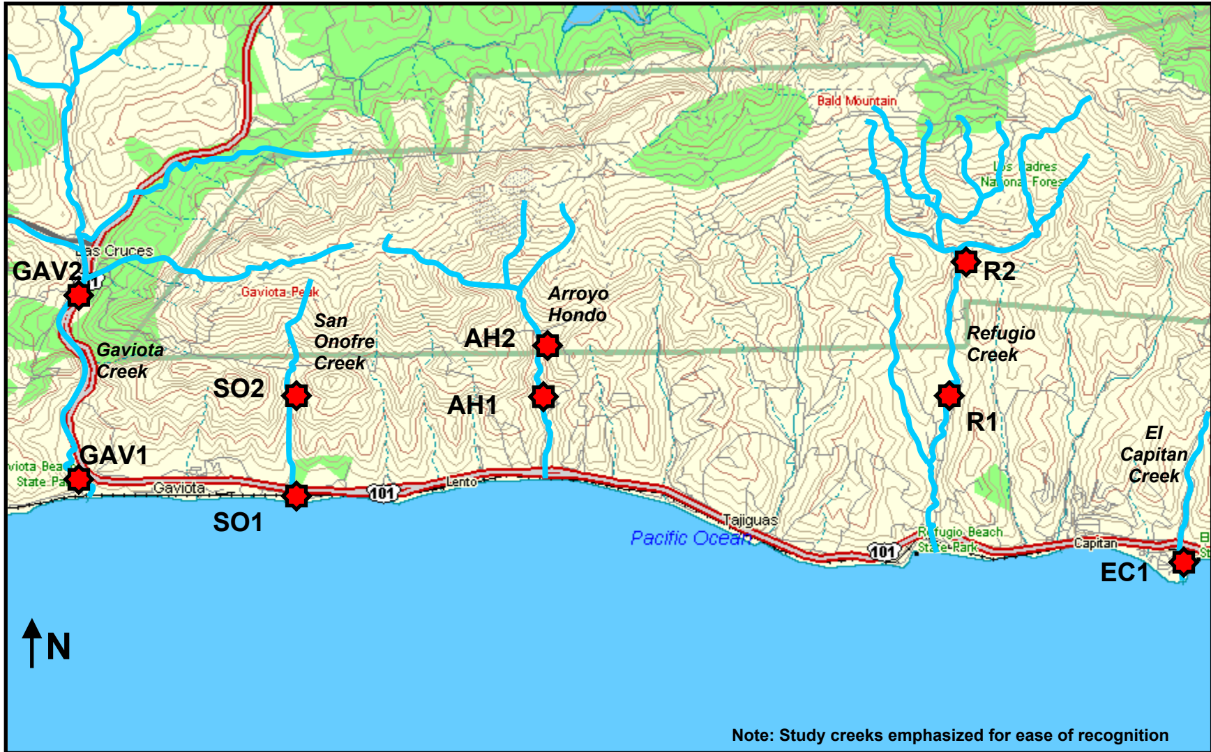
FIGURE 2: GAVIOTA COAST STUDY REACHES
