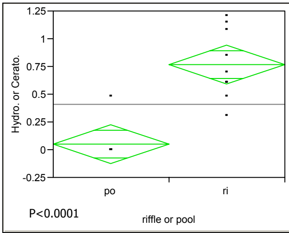
FIGURE 16: SELECTED RIFFLES VS. POOLS T-TESTS
