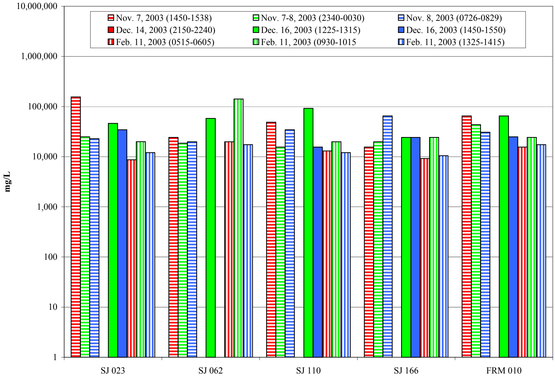
Figure D-3. Enterococcus
