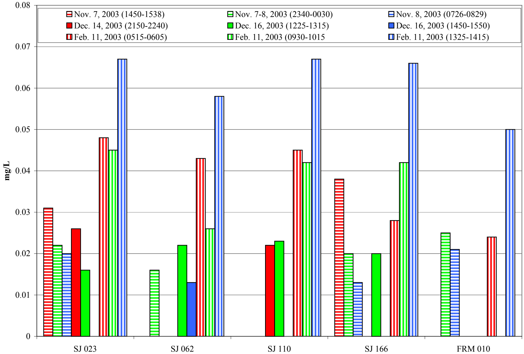
Figure D-4. Glyphosate
