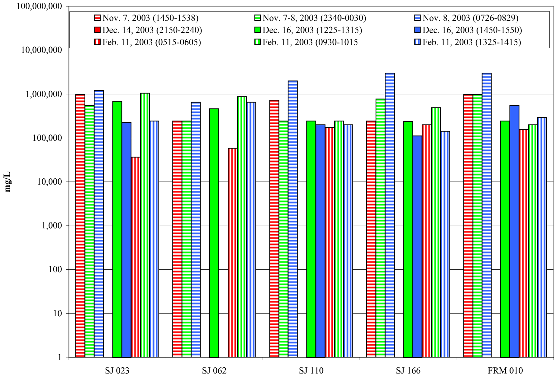
Figure D-1. Total Coliform
