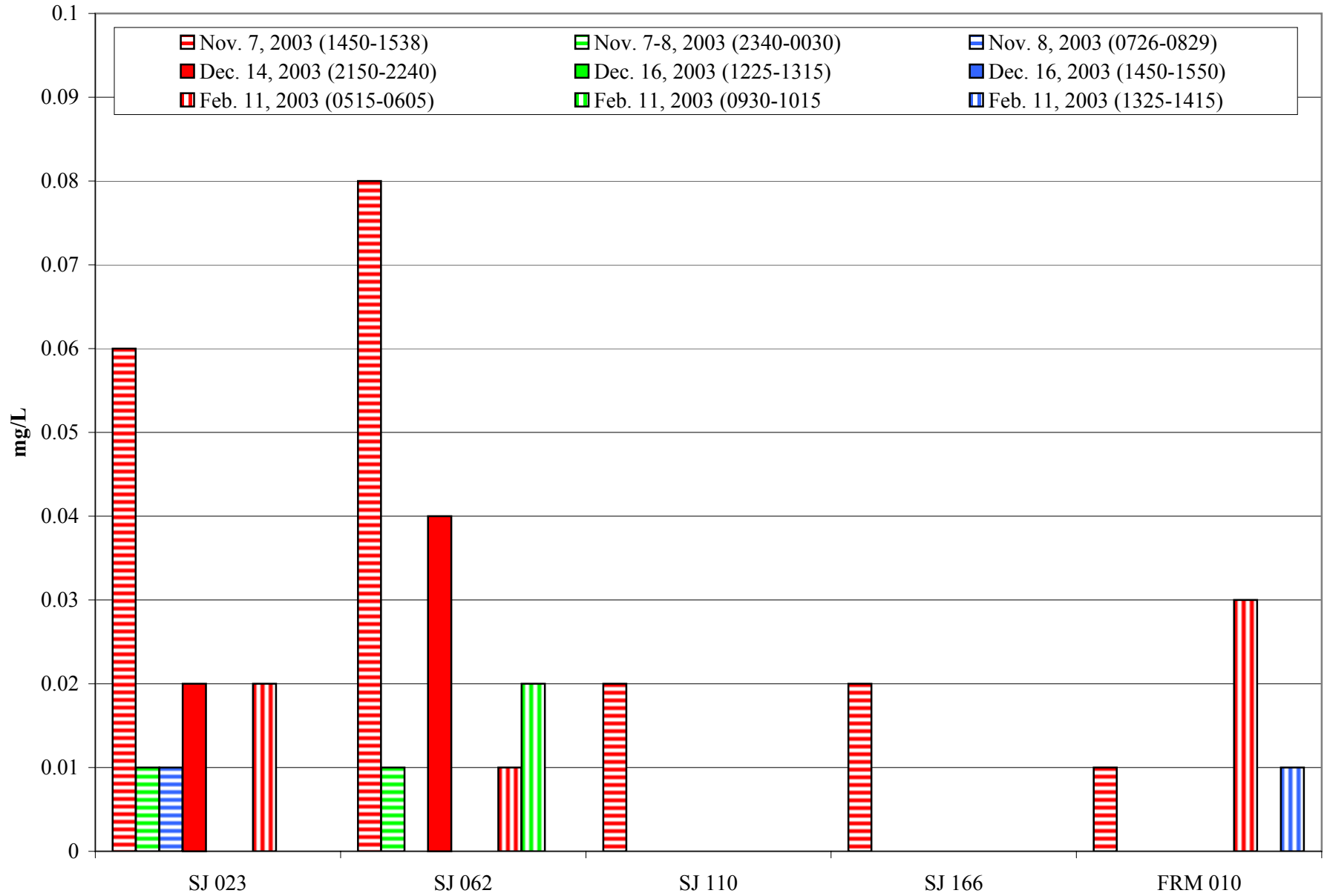
Figure D-7. Zinc
