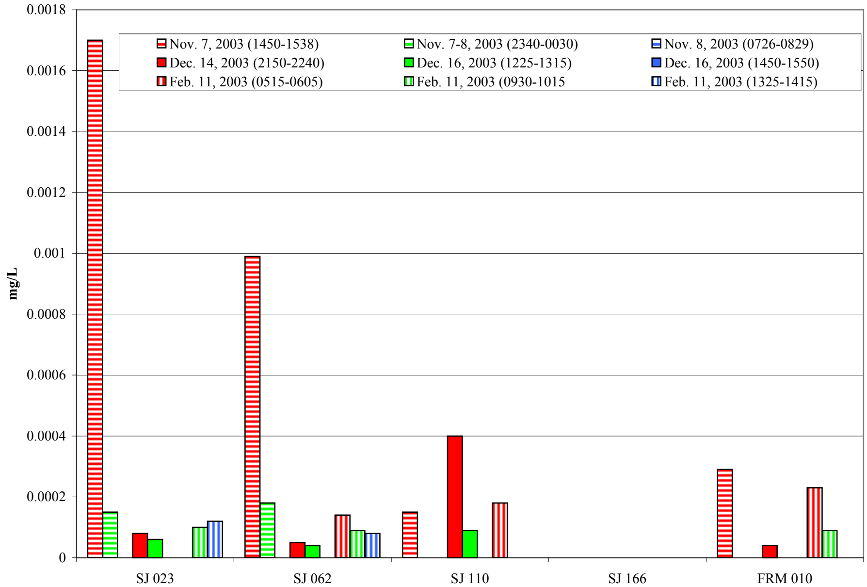
Figure D-5. Diazinon
