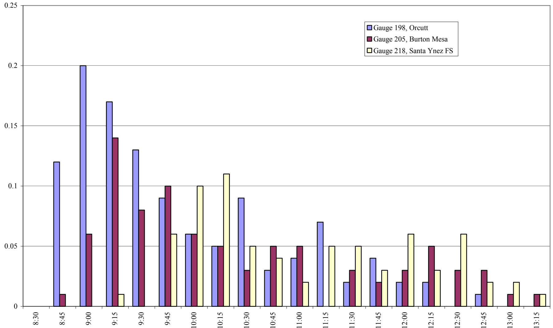
Figure B-3b. Rainfall for December 16, in inches (North County creeks sampled 0940-1210)
