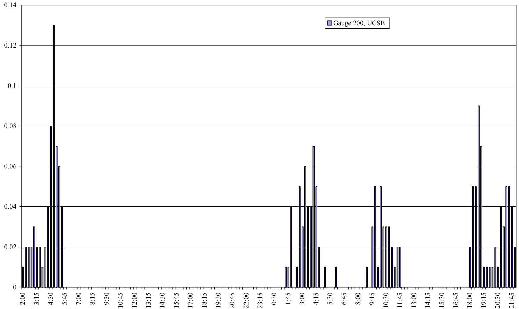
Figure B-4a. Rainfall for February 11-12, in inches (San Jose creek sampled 0515-1415)
