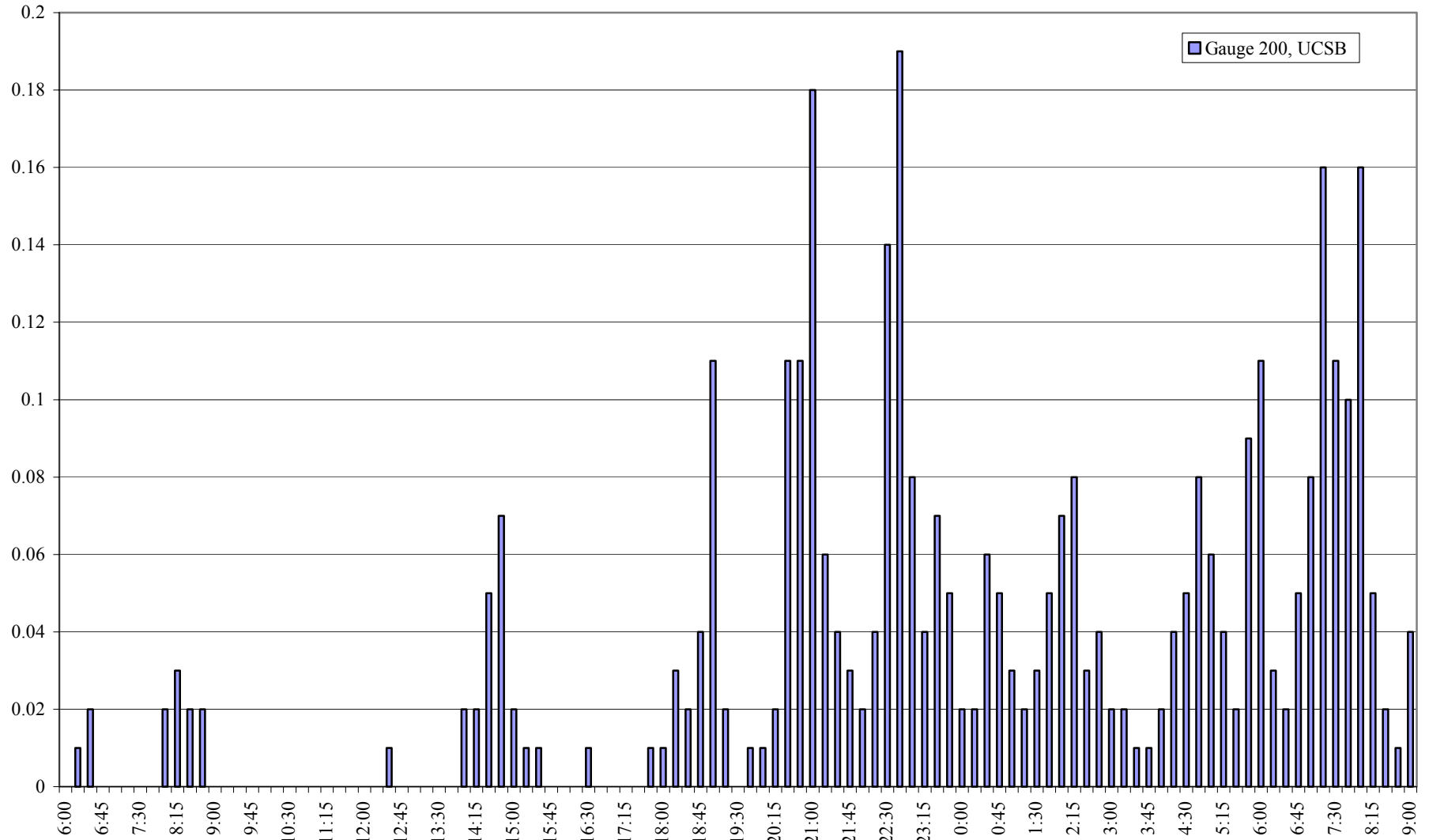
Figure B-2a. Rainfall for November 7-8, in inches (San Jose creek sampled 1450-0829)
