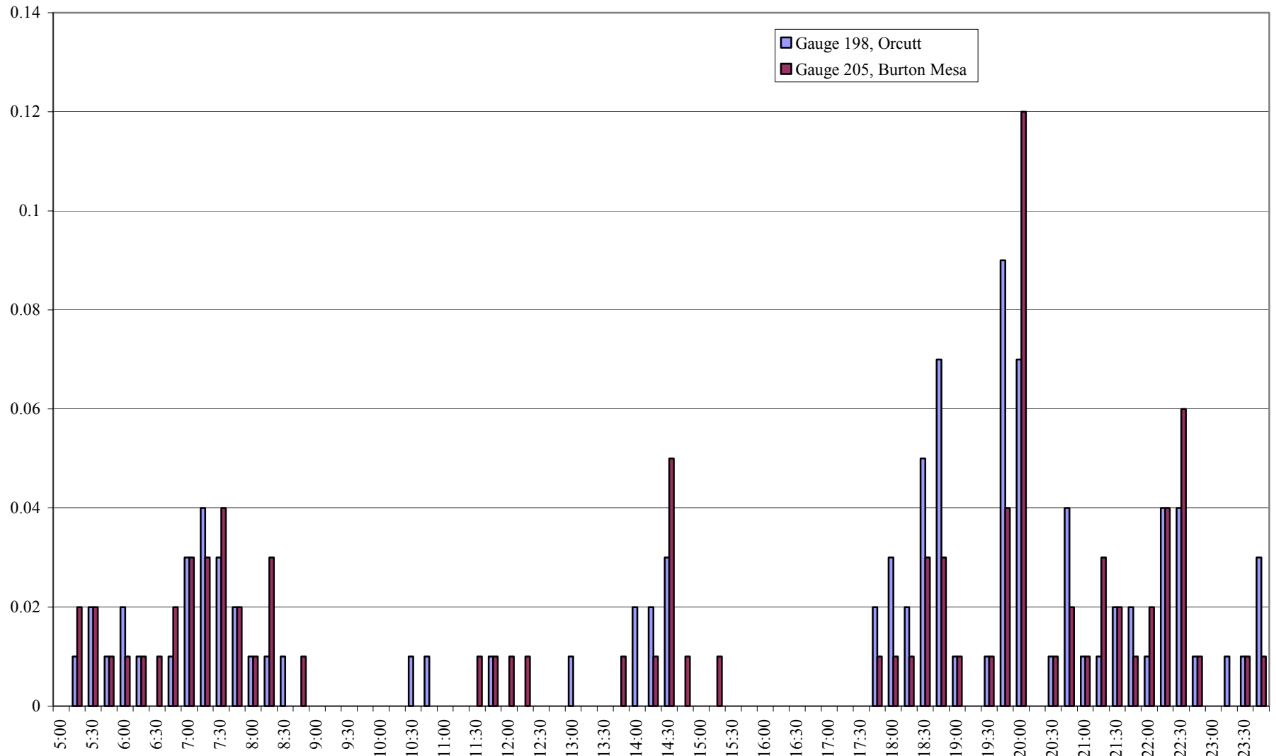
Figure B-2b. Rainfall for November 7-8, in inches (North County creeks sampled 0950 to 2200)
