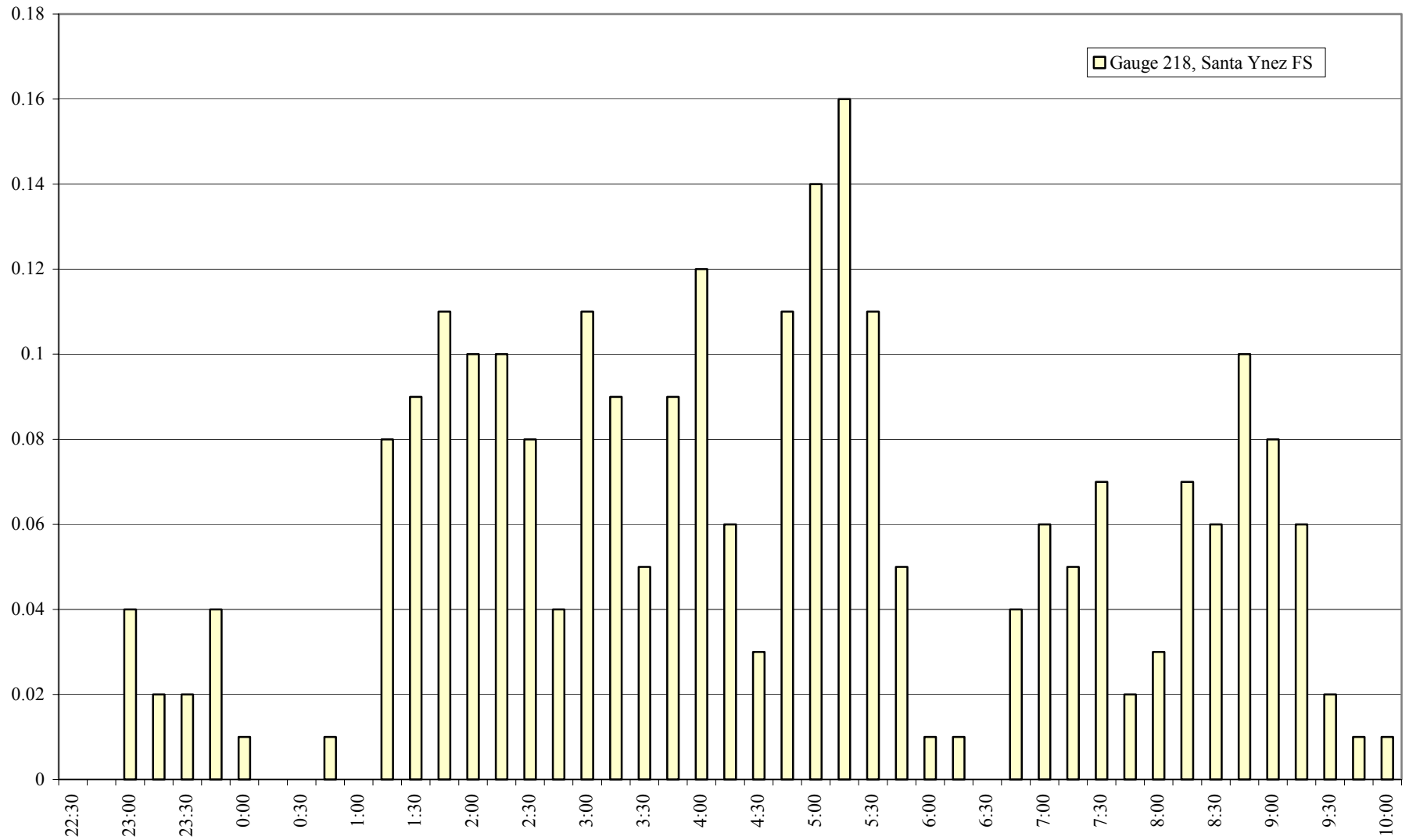
Figure B-6. Rainfall for March 15, in inches (Santa Ynez creeks sampled at 0440)
