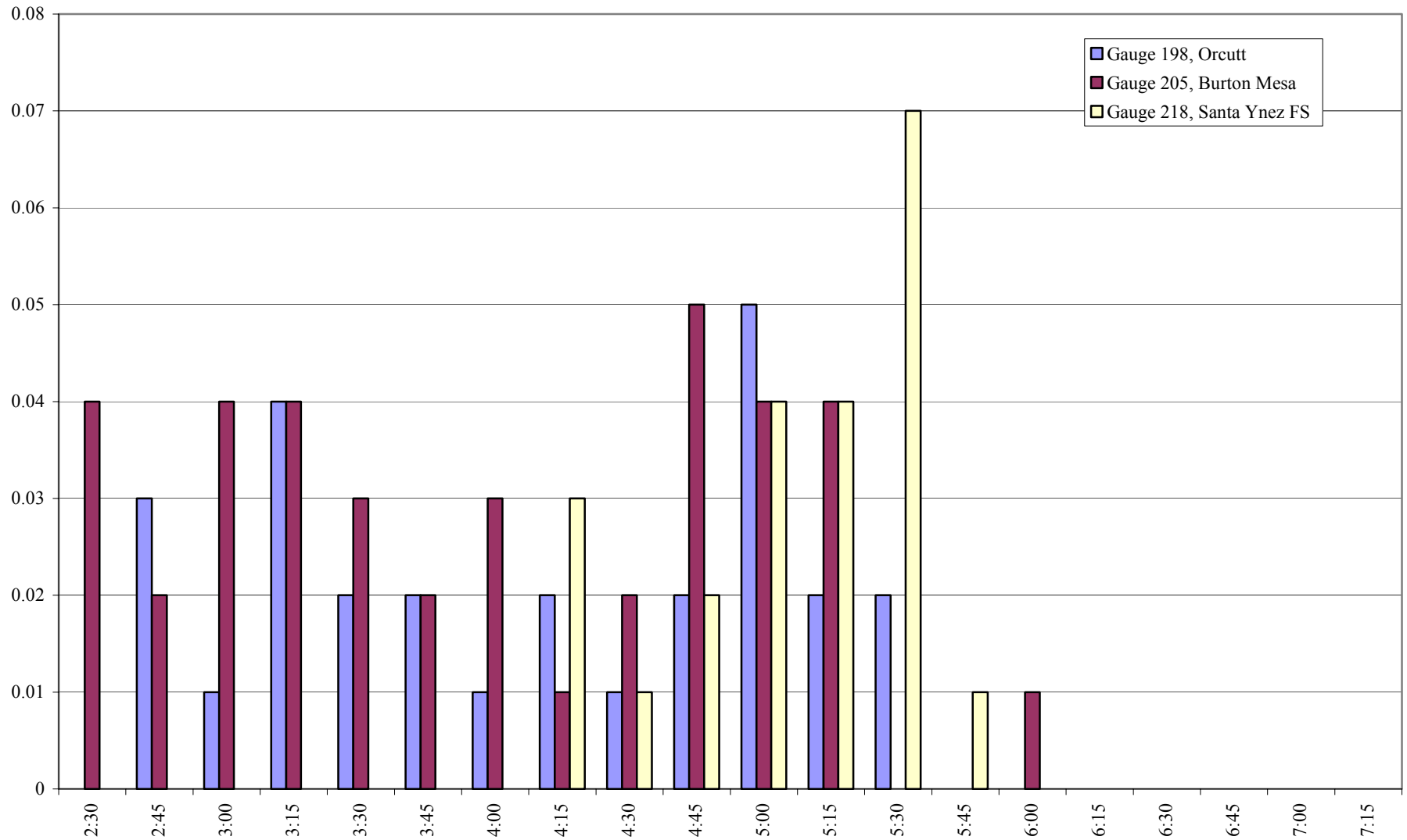
Figure B-4b. Rainfall for February 12, in inches (North County creeks sampled 0500-0700)
