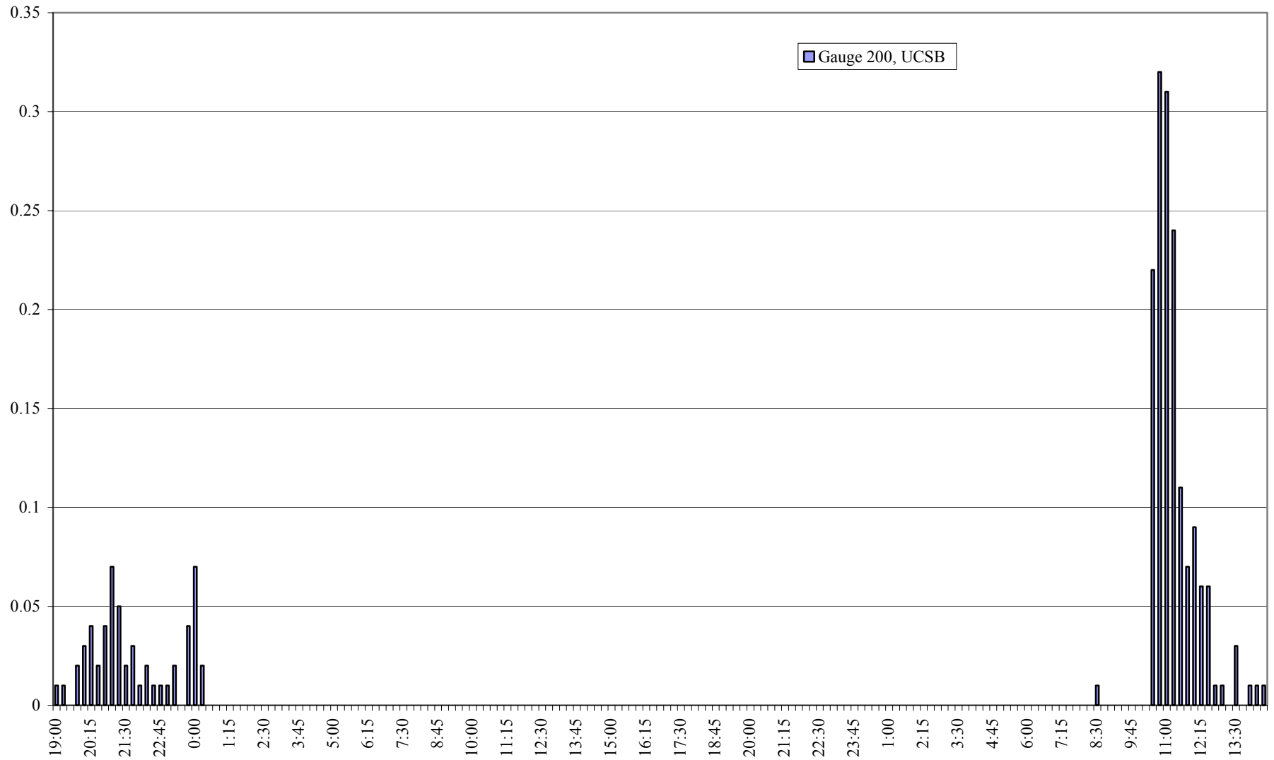
Figure B-3a. Rainfall for December 14-16, in inches (San Jose creek sampled 2150 [12/14]-1550 [12/16])
