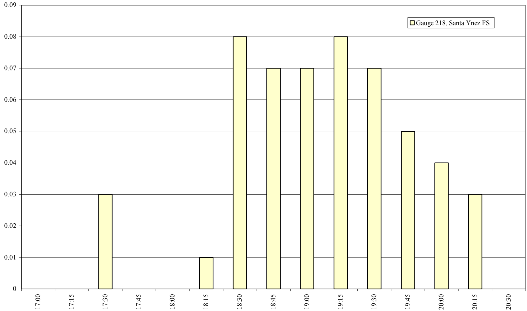
Figure B-5. Rainfall for February 24, in inches (Santa Ynez creeks sampled 1959-2020)
