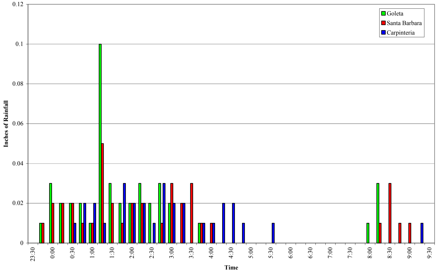
Figure B-4. Rainfall intensities for the February 17, 2002 storm (creeks sampled 1040 to 1540)
