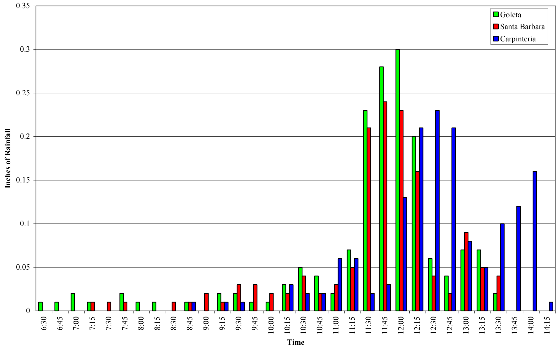
Figure B-3. Rainfall intensities for the November 24, 2001 storm (creeks sampled 1023 to 1625)
